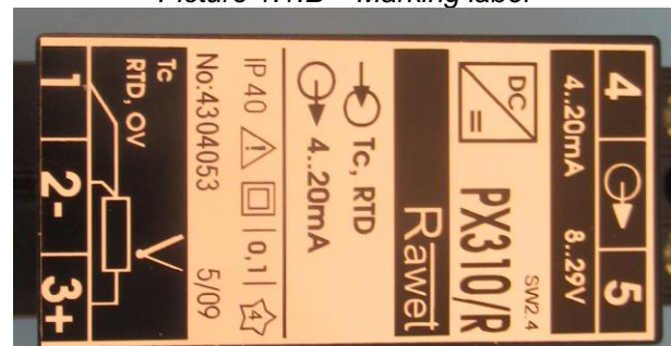
Picture 1.1.B – Marking label
