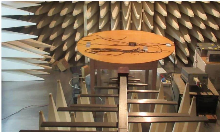
Picture 3.2.A – EUT during testing field immunity
