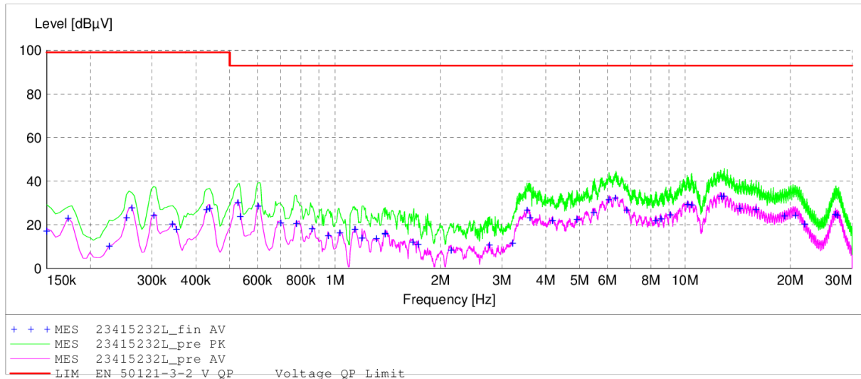
Graph 2.1.B – Conducted terminal voltage according to the ČSN EN 50121-3-2 ed.4, terminal -
