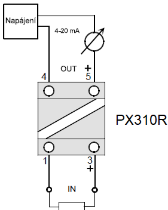
Picture 1.9.A – Block Schematic
