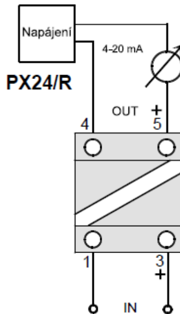
Picture 1.9. – Block Schematic
