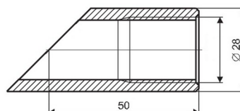
Angled weld-on boss
