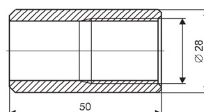
Straight weld-on boss
