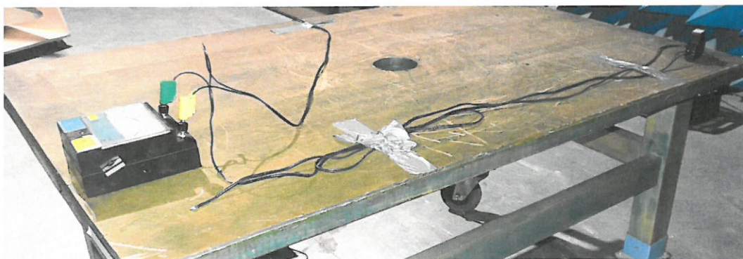
Fig.3 Arrangement of the EUT during the test according to EN 61000-4-3
