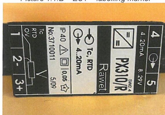
Picture 1.1.B – EUT – labelling marker
