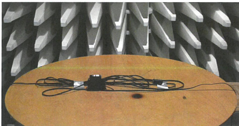
Picture 3.2.A – EUT during the field immunity test
