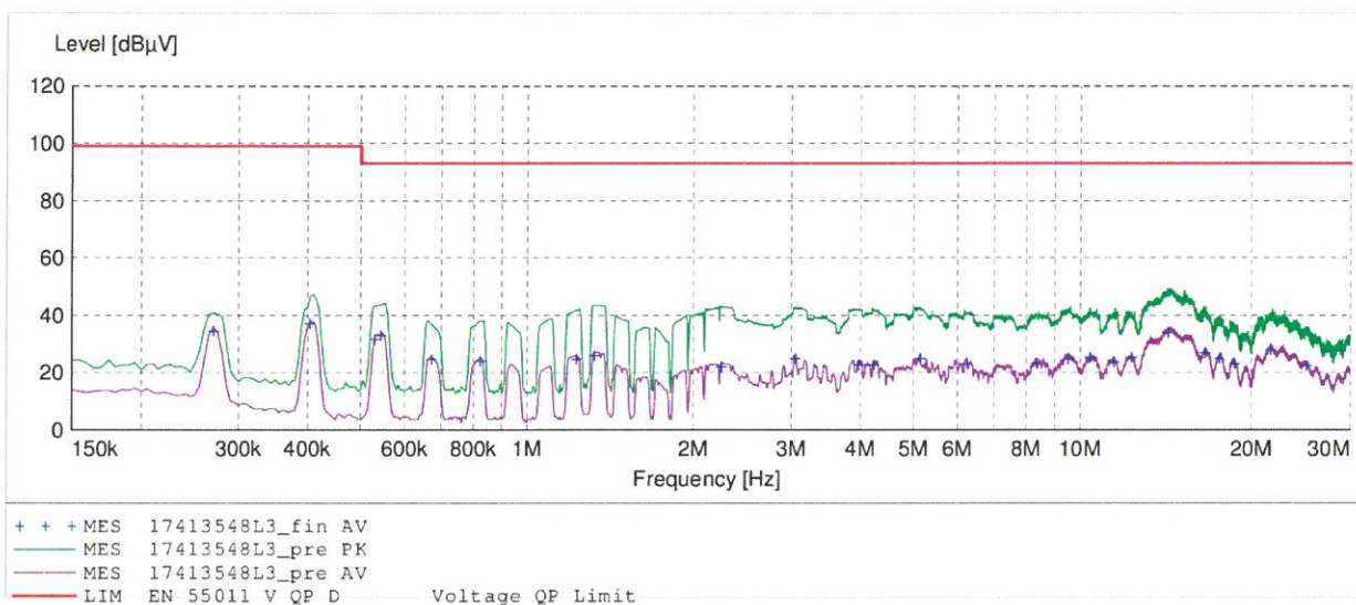
Graph 2.1.B – Conducted terminal voltage ČSN EN 50121-3-2, quasi-peak, terminal -
