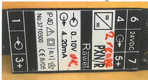
Picture 1.1.B – EUT – labelling marker
