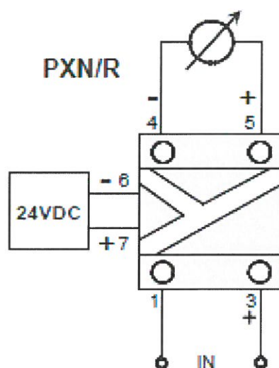
Picture 1.8.A – block diagram
