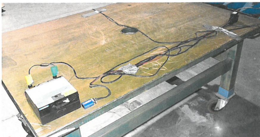
Fig.3 Arrangement of the EUT during the test according to EN 61000-4-3
